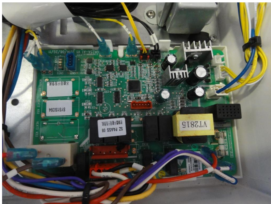
Main board
